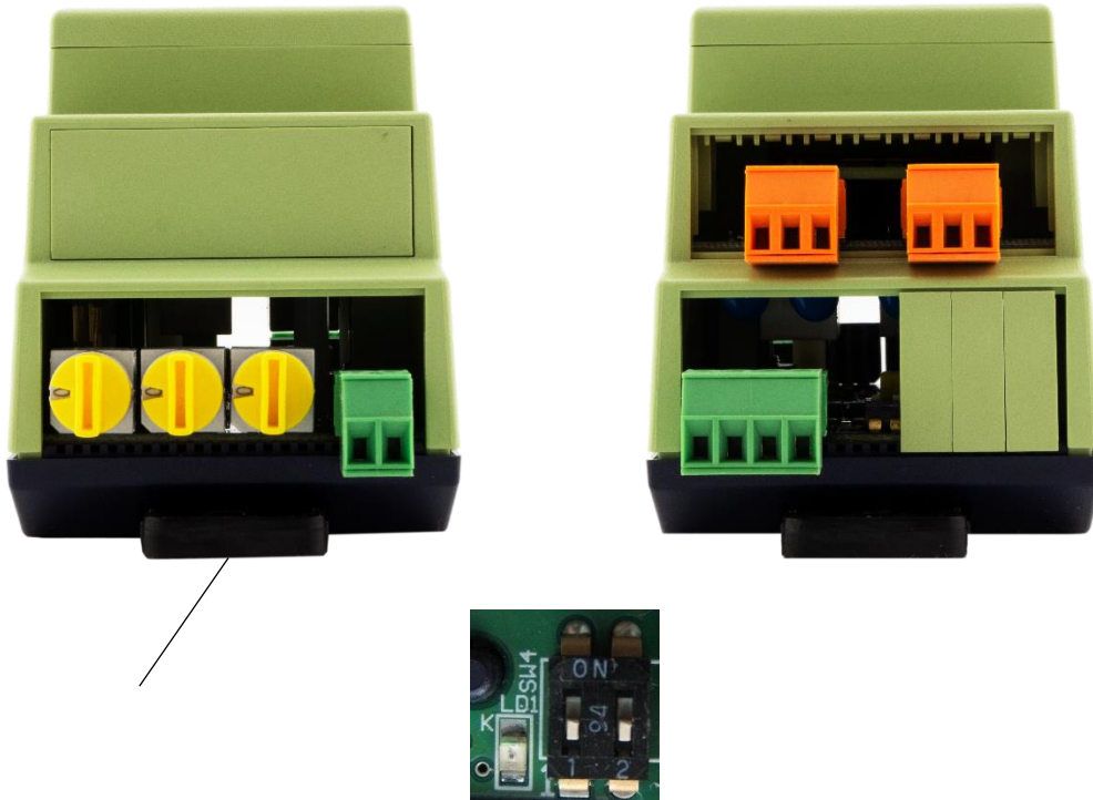
Network LED and Channel Selector Switch
