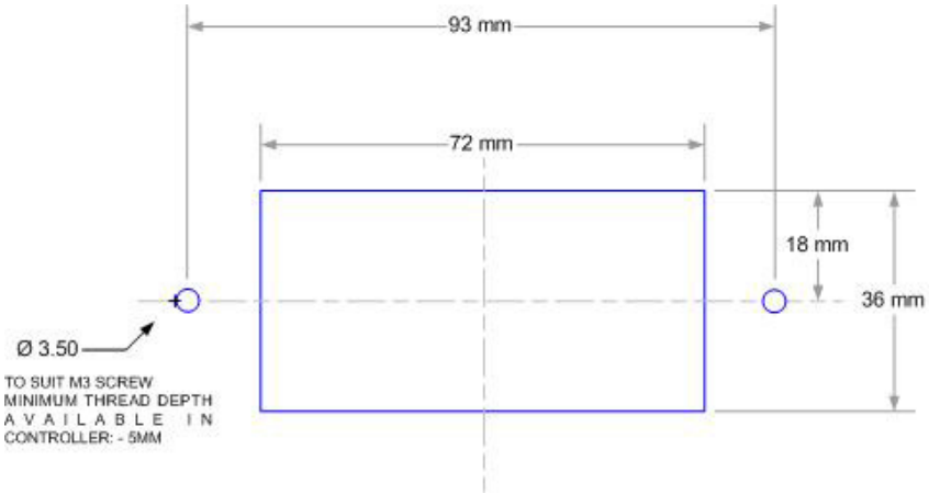
Panel Cut-out
